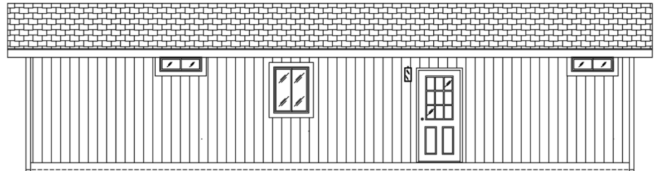
BACK SIDEWALL
